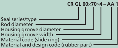
Designation codes for rod seals series GL
