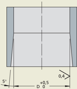
Calibration sleeve
