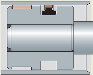
Double-acting piston seal type GHT
