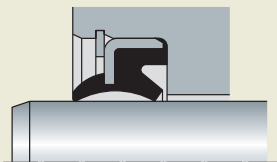
Double-acting wiper seal type SCB with retainer ring type SP
