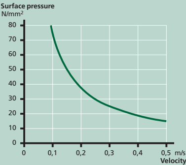
pv diagram for guide rings of phenolic/fabric at 70 °C
