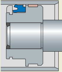
Single-acting piston seal type SAARR
