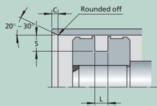
Housing groove section
