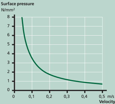
pv diagram for guide rings of PTFE MS-292 at 70 °C
