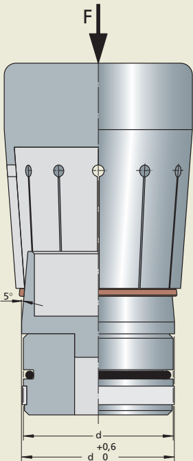
Assembly tool
