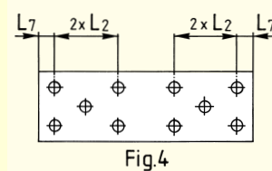
Layout of the standard attaching holes in the lower section
