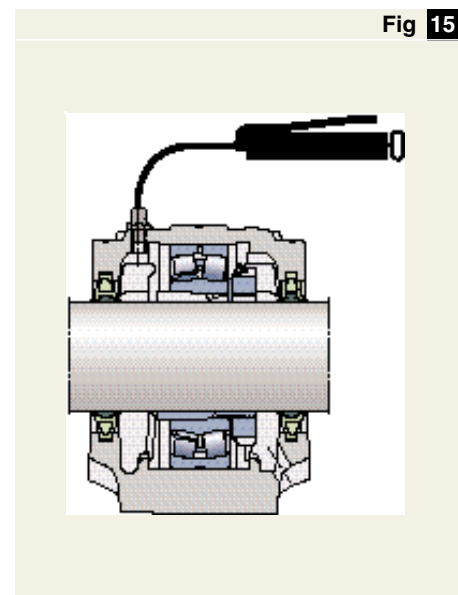
Housing with grease escape hole
